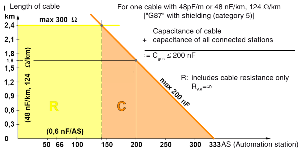
Fig. 5 novaNet performance chart
