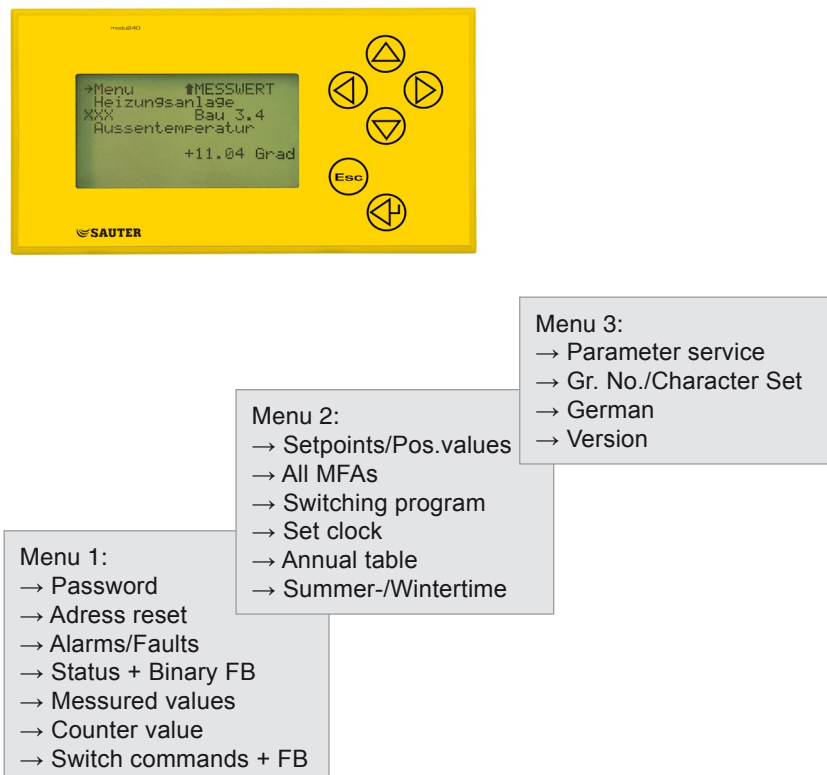
Fig. 2 Local operating unit, modu240
