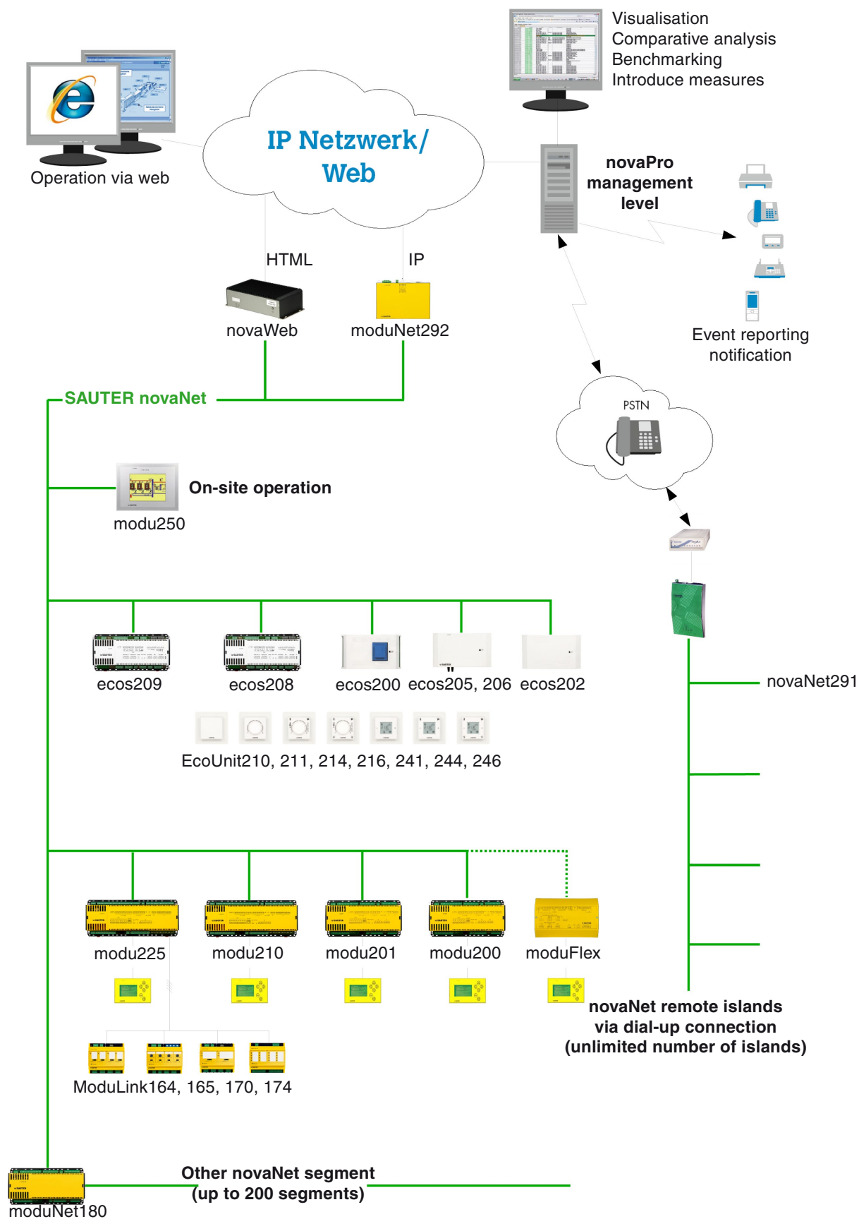
Fig. 1 System overview
